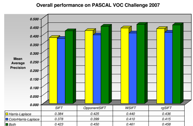
Figure 3. Mean Average Precision performance over all 20 object categories on the PASCAL VOC Challenge 2007 dataset.
