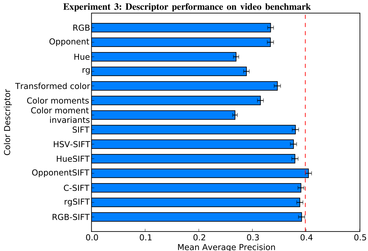
Fig. 8. Evaluation of color descriptors on a video benchmark, the Mediamill Challenge [22], averaged over 39 object and scene categories. Error bars indicate the standard deviation in mean average precision, obtained using bootstrap. The dashed line indicates the lower bound of the OpponentSIFT confidence interval.
