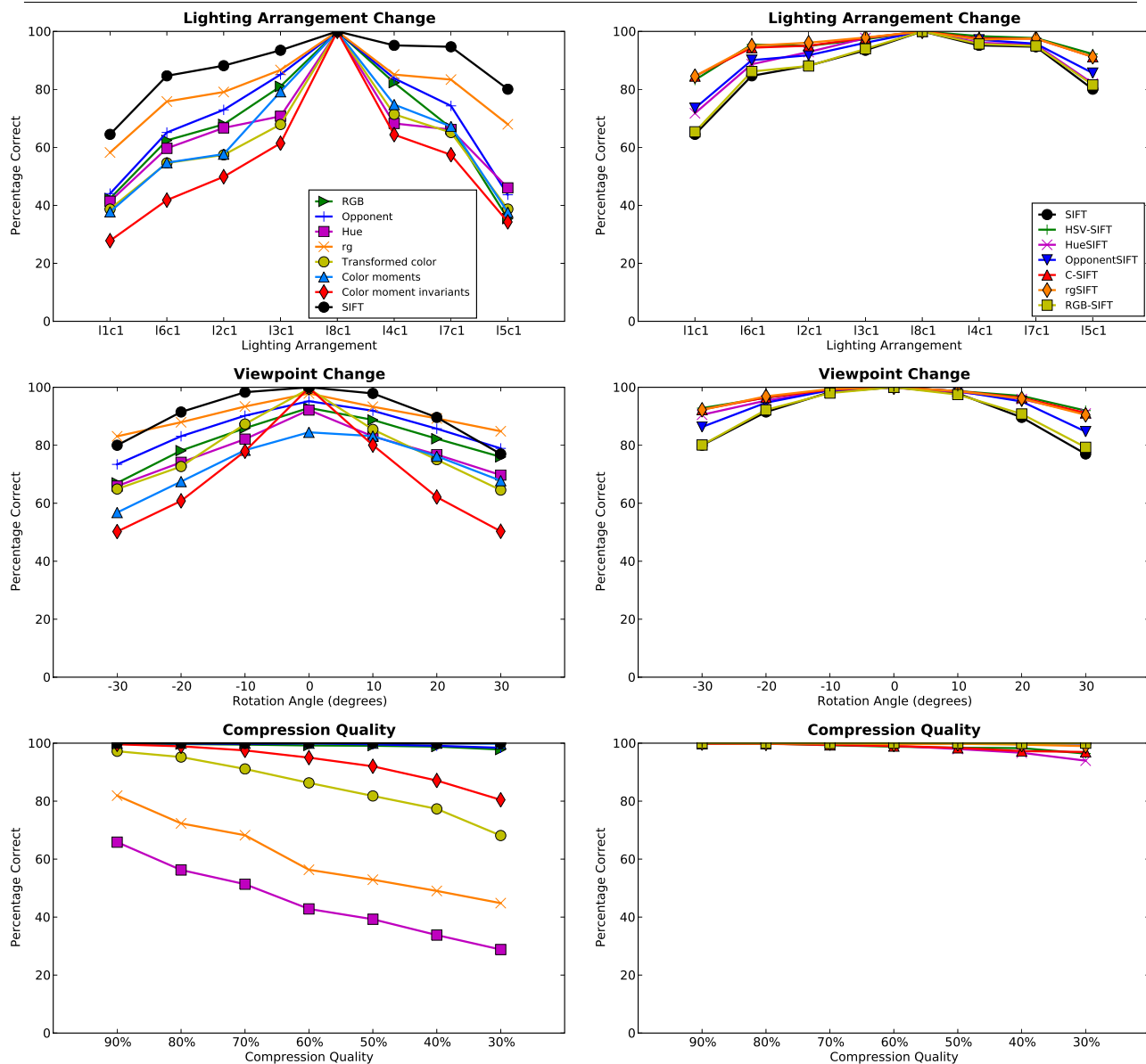
Fig. 5. For completeness, this figure contains the results for color descriptors under different lighting arrangements at increasingly oblique angles (between one and three of the lights around the object are on, introducing selfshadowing for up to half of the object), different viewpoint angles and different degrees of JPEG compression, averaged over 1000 objects from the ALOI dataset [20]. Performance is measured using the percentage of correctly identified objects. For clarity of presentation, the results have been split into two parts. To allow for easier comparison, SIFT is shown in both the graphs on the left and the graphs on the right.
