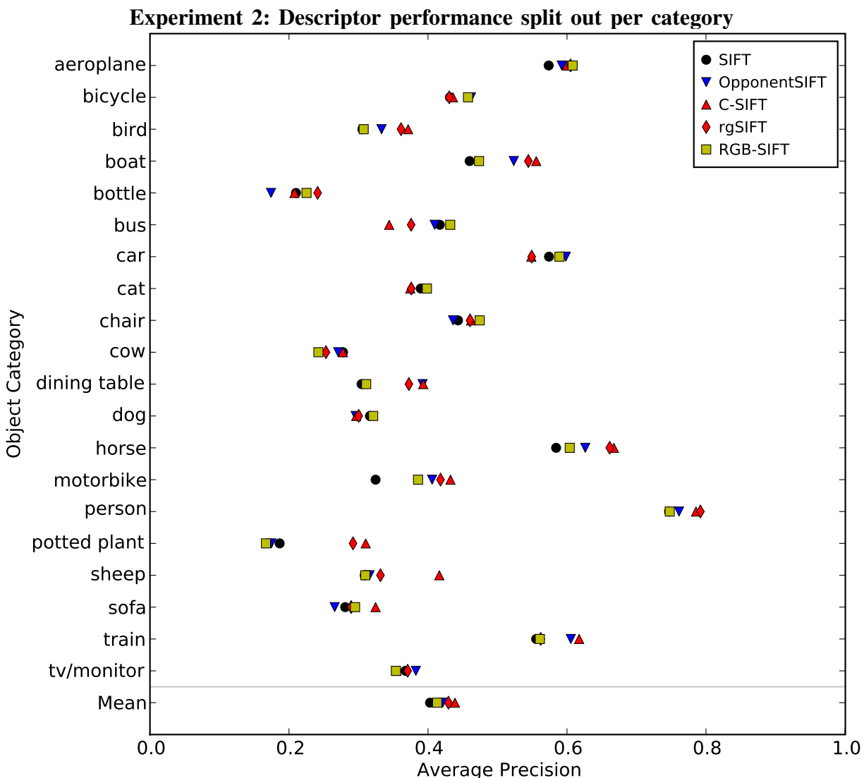
Fig. 7. Evaluation of color descriptors on an image benchmark, the PASCAL VOC Challenge 2007, split out per object category. SIFT and the best four color SIFT variants from figure 6 are shown.
